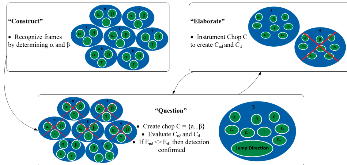
Figure 3.1: REDIR concept through the Data/Frame sensemaking process.
